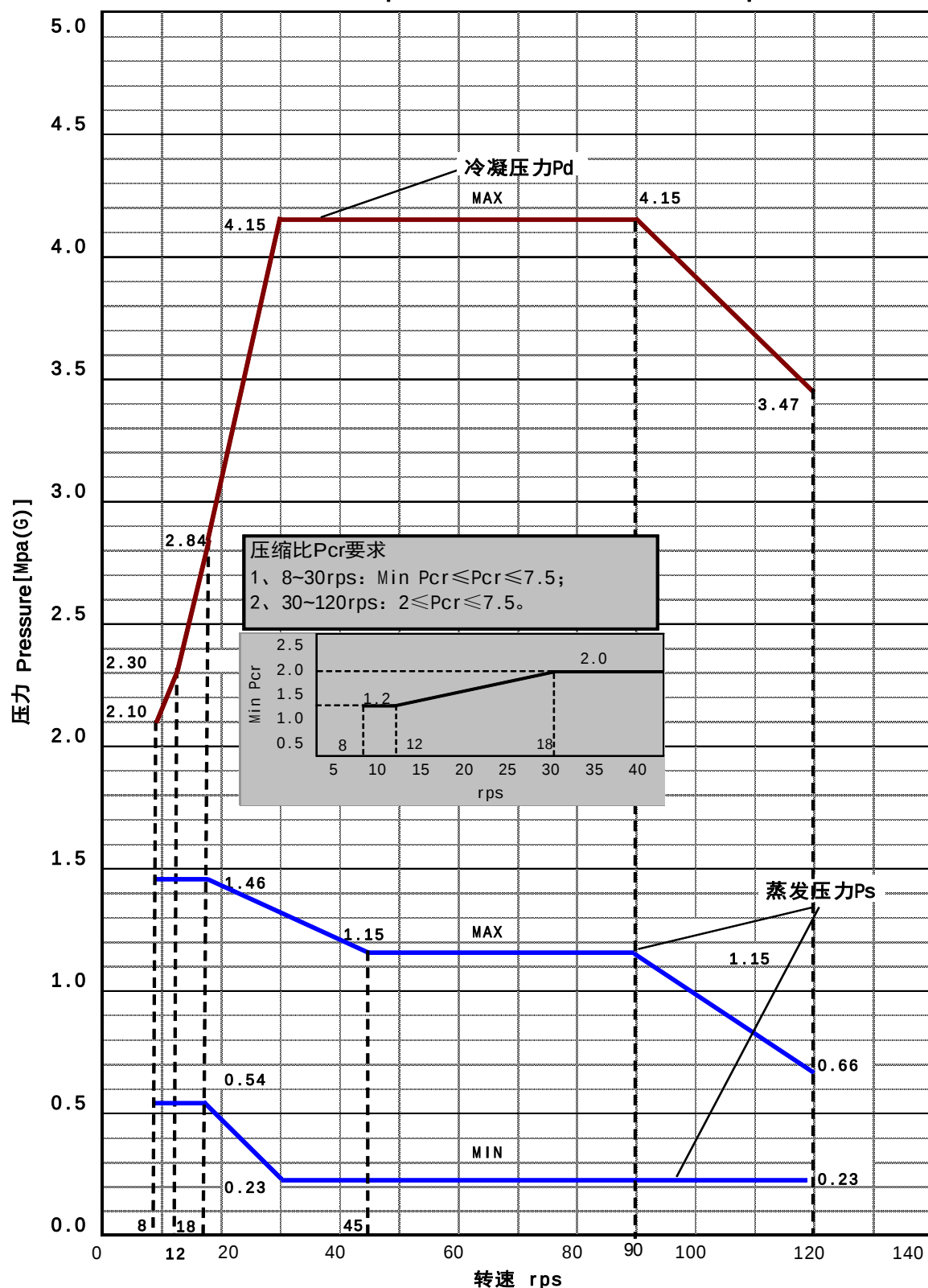
压缩机运行范围 Operation Limitation of Compressor
